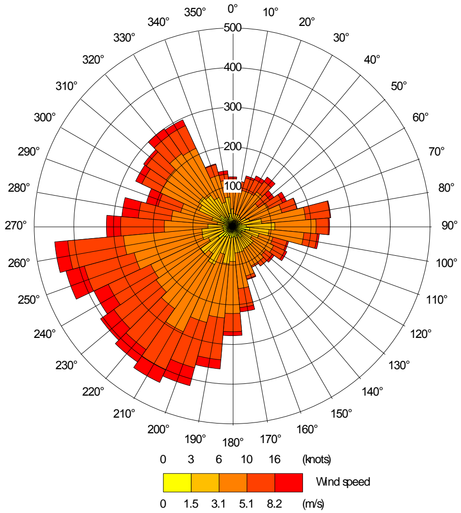
Figure 14.1: Wind Rose
